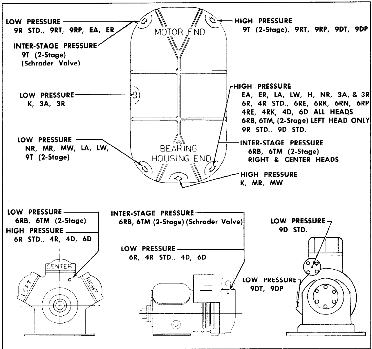
HEAD POSITIONS WHEN VIEWED FROM BEARING HOUSING END OF COMPRESSOR
