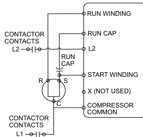
Figure 1 - Wiring Diagram
